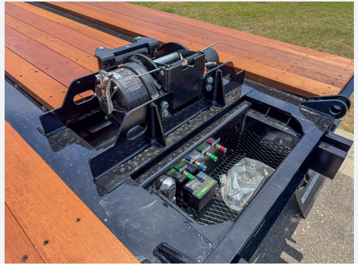
Gooseneck-mounted hydraulic power unit
