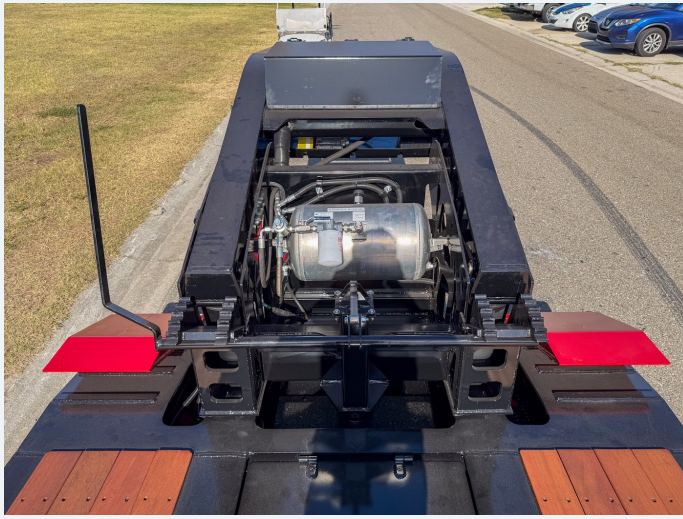
Gooseneck-mounted hydraulic power unit
