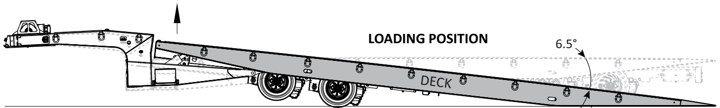
The axles travel forward and allow the deck to rise and allow for a very low 6.5 degree load position.
