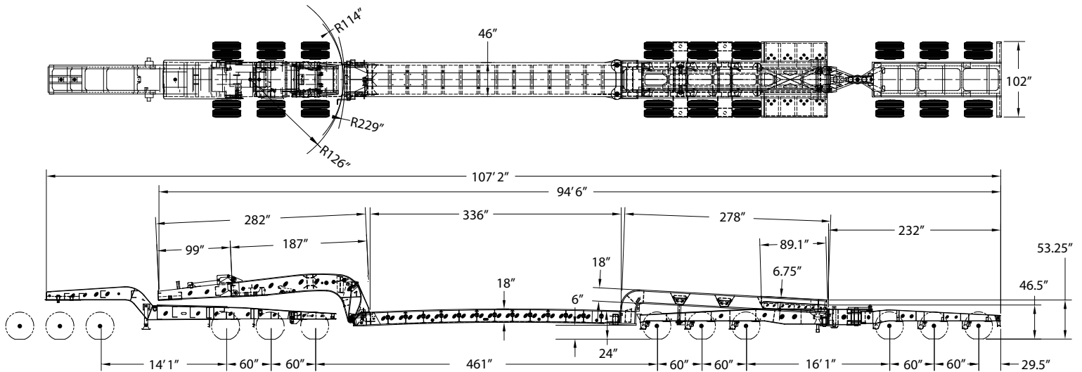
Trailer Model: GTBN803-67-28-HGG
