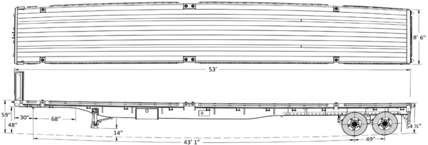
Trailer Model: GTFF402-48
