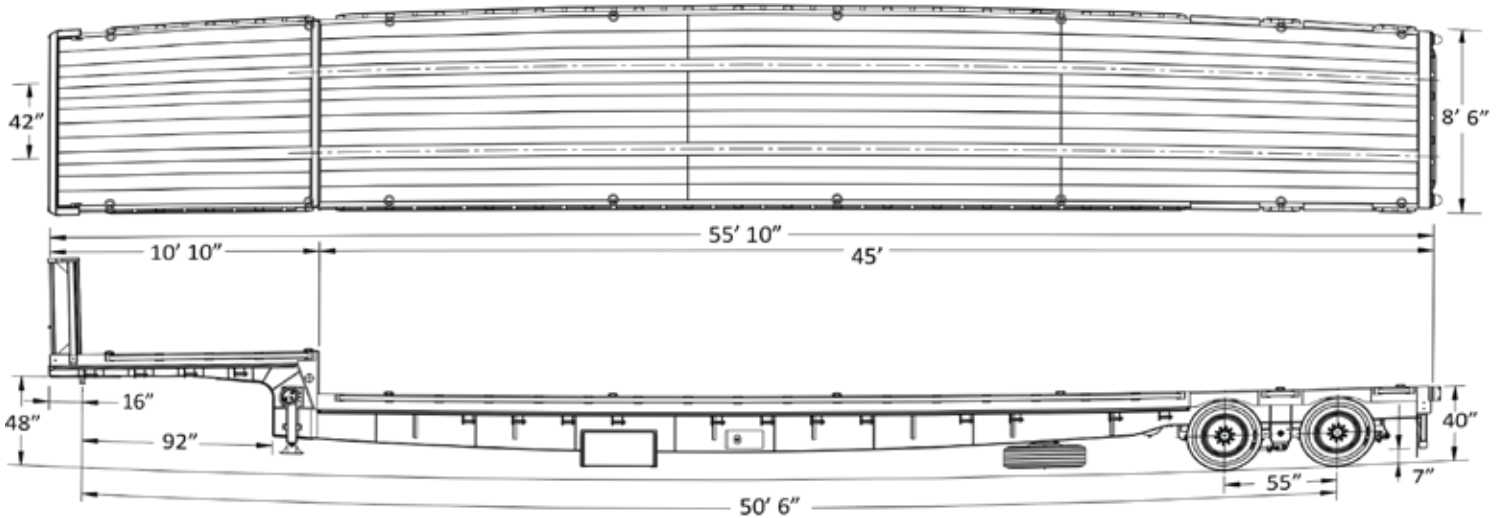
Trailer Model: GTFS402-56-45
